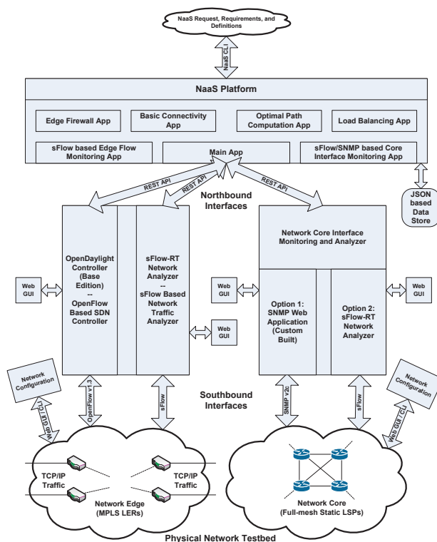
Fig. 3: The Proof-of-Concept design of our architecture.
