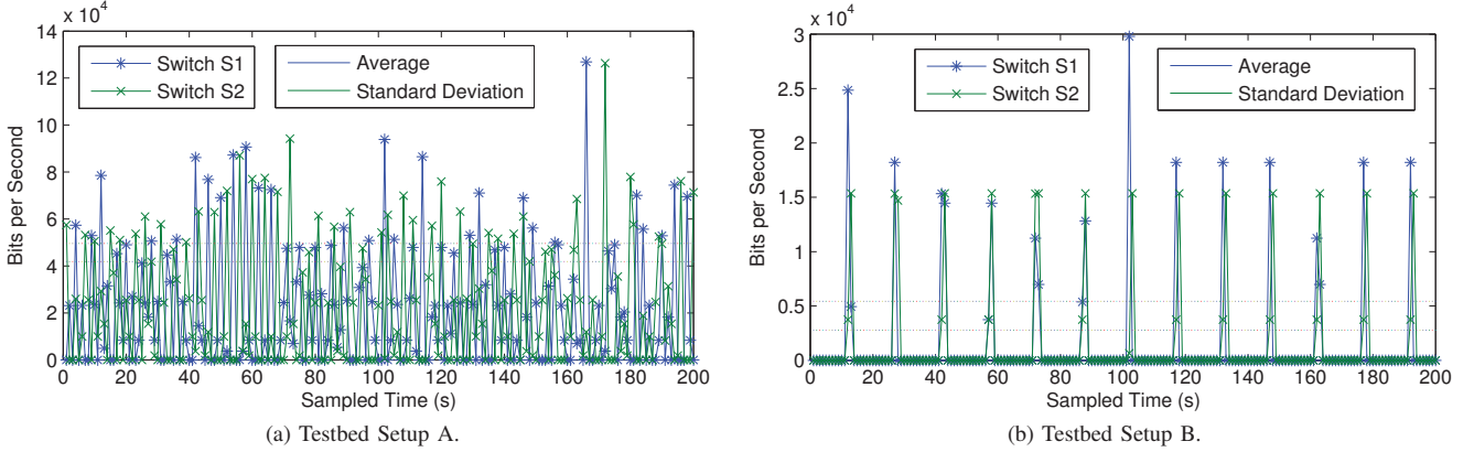
Fig. 6: OpenFlow protocol traffic load samples at the OpenDaylight Controller in the PoC physical network testbed.
