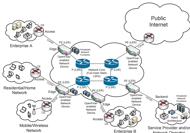
Fig. 2: Our proposed SDN-based architecture.
