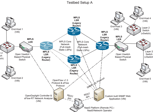
Fig. 4: Testbed Setup A with Juniper (M10i) legacy routers as the network core MPLS LSRs.
